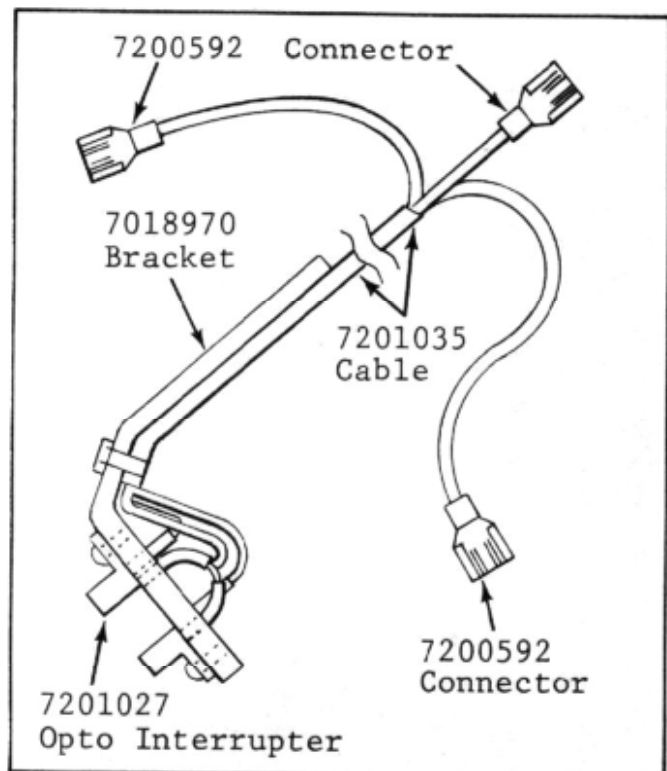
7021355 - Shuttle Clock Assy (Complete)
