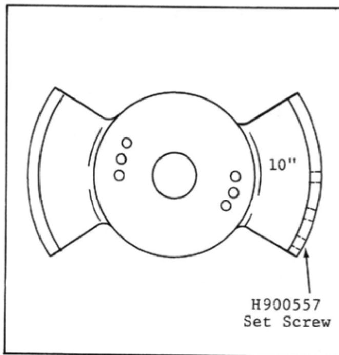
7008345 - Vacuum Shoe
